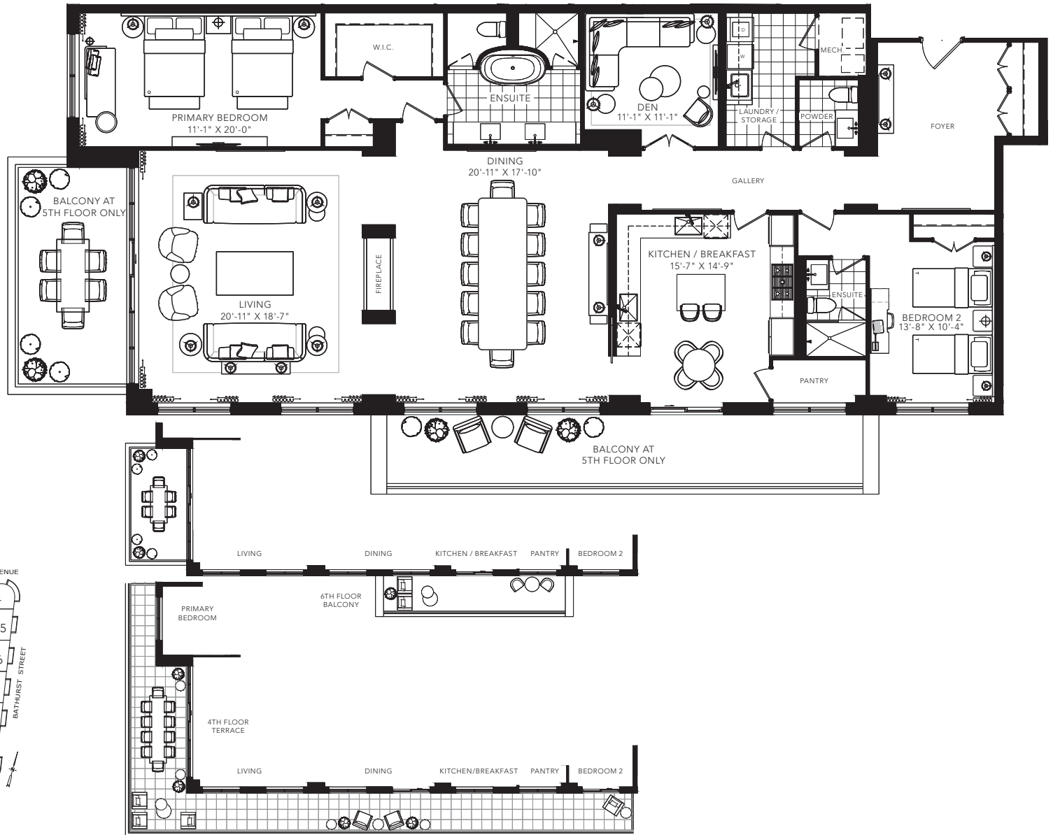
FLOOR 6
